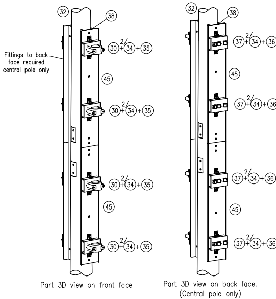
3D VIEWS ON CABLE GUARD BACK PLATE (CABLE GUARDS OMITTED FOR CLARITY) Scale 1:25
